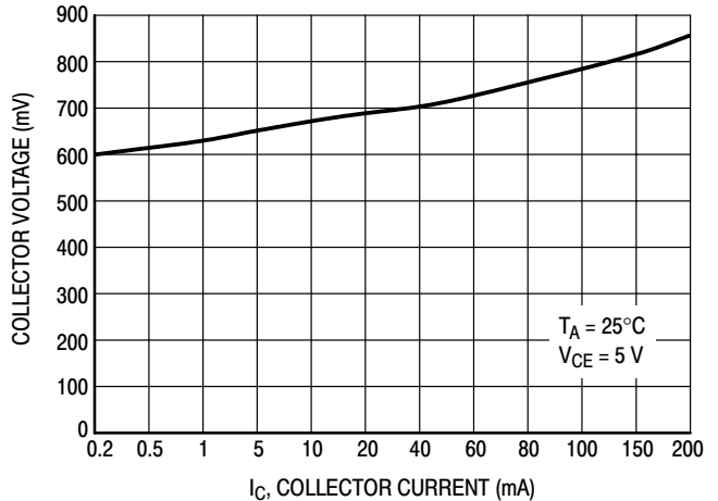
Figure 4. On Voltage
